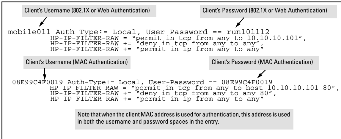
Figure 6-6. Example of Configuring the FreeRADIUS Server To Support ACLs for the Indicated Clients
